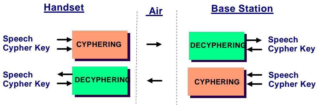
Figure 10. The DECT cyphering function
