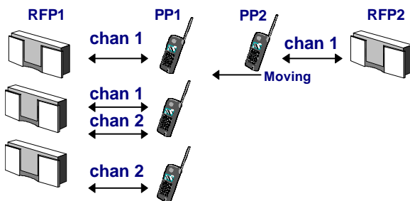
Figure 6. The DECT intracell handover function
