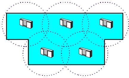
Figure 2. The pico-cellular structure of the DECT access network
